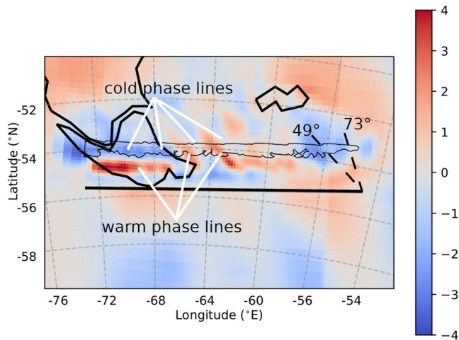
Figure 3. Temperature perturbation component at 10-km altitude of the Gimballed Limb Observer for Radiance Imaging of the Atmosphere (GLORIA) tomographic field. The retrieval was computed using data only from the southern leg (thick black line). Using both the northern and southern legs in a combined tomographic retrieval created artifacts due to nonsymmetrical tangent point distribution. A retrieval using only the northern leg produced a gravity wave (GW) field similar to the southern leg. Black solid lines indicate the Patagonia coastline and the straight white solid lines point to different phase fronts. The region encircled by the thin black line indicates our tangent point region for this altitude, which is our region of trust (Section 2.1.1). The dashed black lines indicate the maximum and minimum GLORIA line-of-sight angle discussed in Figure 4.
