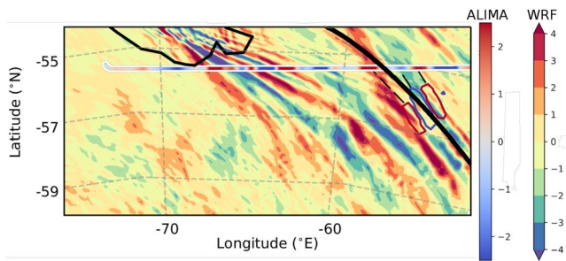
Figure 6. The forward raytrace (bold black line) of the Gimbal Limb Observer for Radiance Imaging of the Atmosphere observed gravity wave (GW) overlaid with WRF and Airborne Lidar for the Middle Atmosphere (ALIMA) data. All data are valid for 27-km altitude. The background data are WRF data while the red and blue lines with the white border represents ALIMA data on the southern flight track after the upward propagating waves were selected with a wavelet transform (Section 2.1.2). The red and blue contour lines are the reconstructed warm and cold phases of the gravity wave (GW) suggested by GROGRAT along the ray path. The GROGRAT reconstructed GW is valid at the respective location and at 27 km. The reconstructed GWs and WRF data are both valid for 12 September 06:00. To guide the eye, the black-dashed lines create a link between GROGRAT reconstruction and the ALIMA track, which shows that the phase fronts of the GW match well. The plot is exclusively used to match the GW structure and validate GROGRAT versus ALIMA. Note that the temperature (in K) scale is different for WRF and ALIMA—the wavelet transform would cause the ALIMA temperature amplitude to be lower than the actual amplitude (Section 2.1.2).
