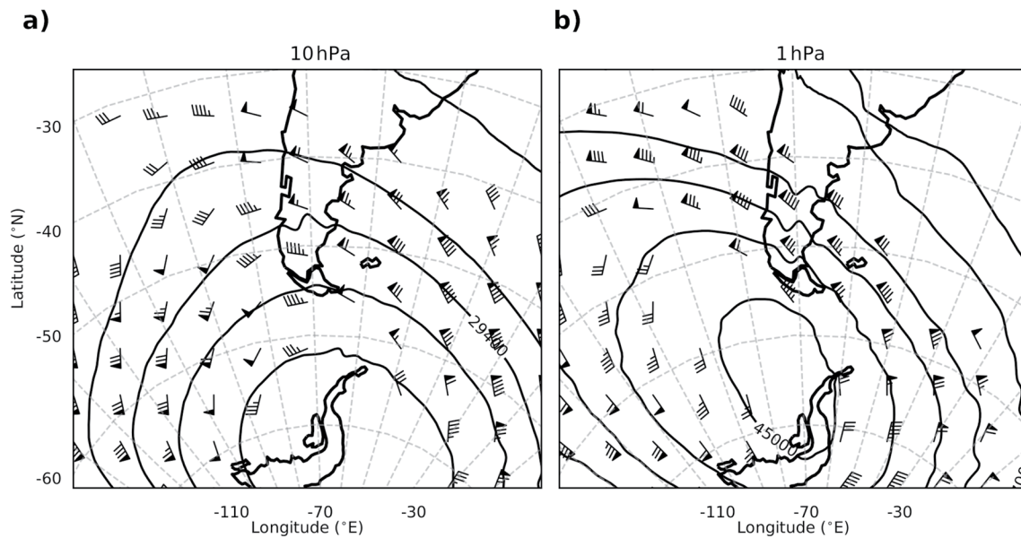
Figure 2. Stratospheric synoptic situation at 10 hPa (a) and 1 hPa (b) on 12 September at 03:00 as indicated by ERA5 (corresponding to ~30-km and 50-km altitudes). Black lines and wind barbs are similar to Figure 1. Note the displaced polar vortex with its center located at 70°S 60°W at 10 hPa and 65°S 75°W at 1 hPa.
