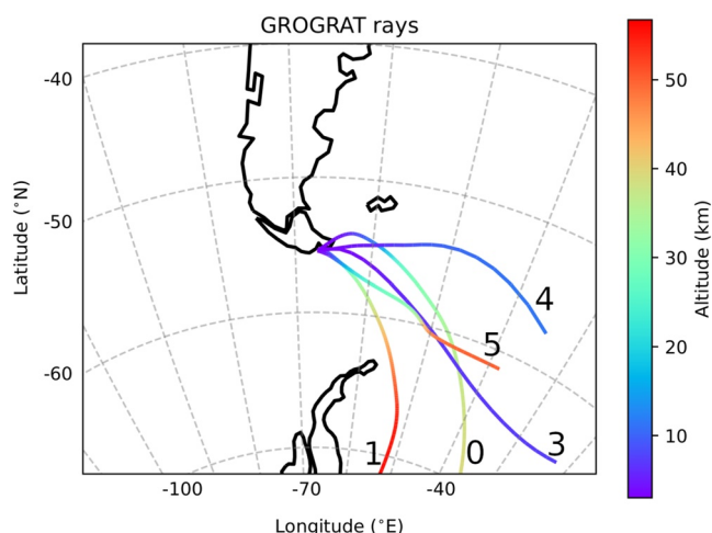
Figure 13. GROGRAT experiments during forward tracing of the Gimbalbed Limb Observer for Radiance Imaging of the Atmosphere observed gravity wave (GW; shown in Figures 3 and 4). Ray #0 shows raytracing using the “normal” setup with 4-D propagation in a high-resolution background. Ray #1 uses the same 4-D propagation setup but uses a background u and v wind, which was multiplied by a factor of 1.5. Ray #2 is not depicted here as it will only show as a dot above the starting location. Ray #3 attempts to reproduce the results of Hasha et al. (2008) and uses a coarse resolution background and only 3-D propagation setup. Ray #4 uses the exact same settings as ray #3 but use background conditions of the “normal” year 2018. Ray #5 uses 4-D propagation settings, but with only a westerly wind with no horizontal gradient. Ray #5 is an attempt to separate the effect of advection from refraction.
